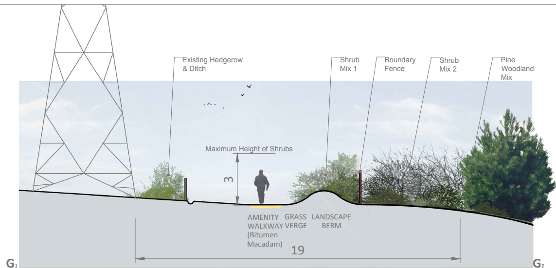
CROSS SECTION G Scale 1:100
