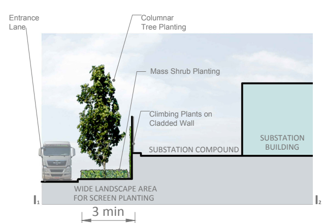
CROSS SECTION I Scale 1:100
