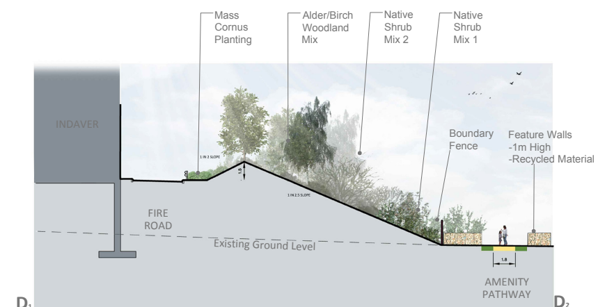
CROSS SECTION D Scale 1:200
