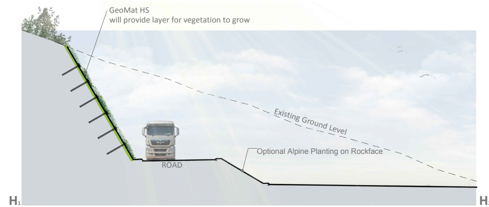
CROSS SECTION H Scale 1:200
