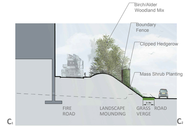
CROSS SECTION C Scale 1:200
